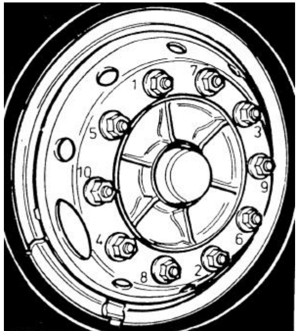
Picture 1. Wheel nut tightening sequence.
